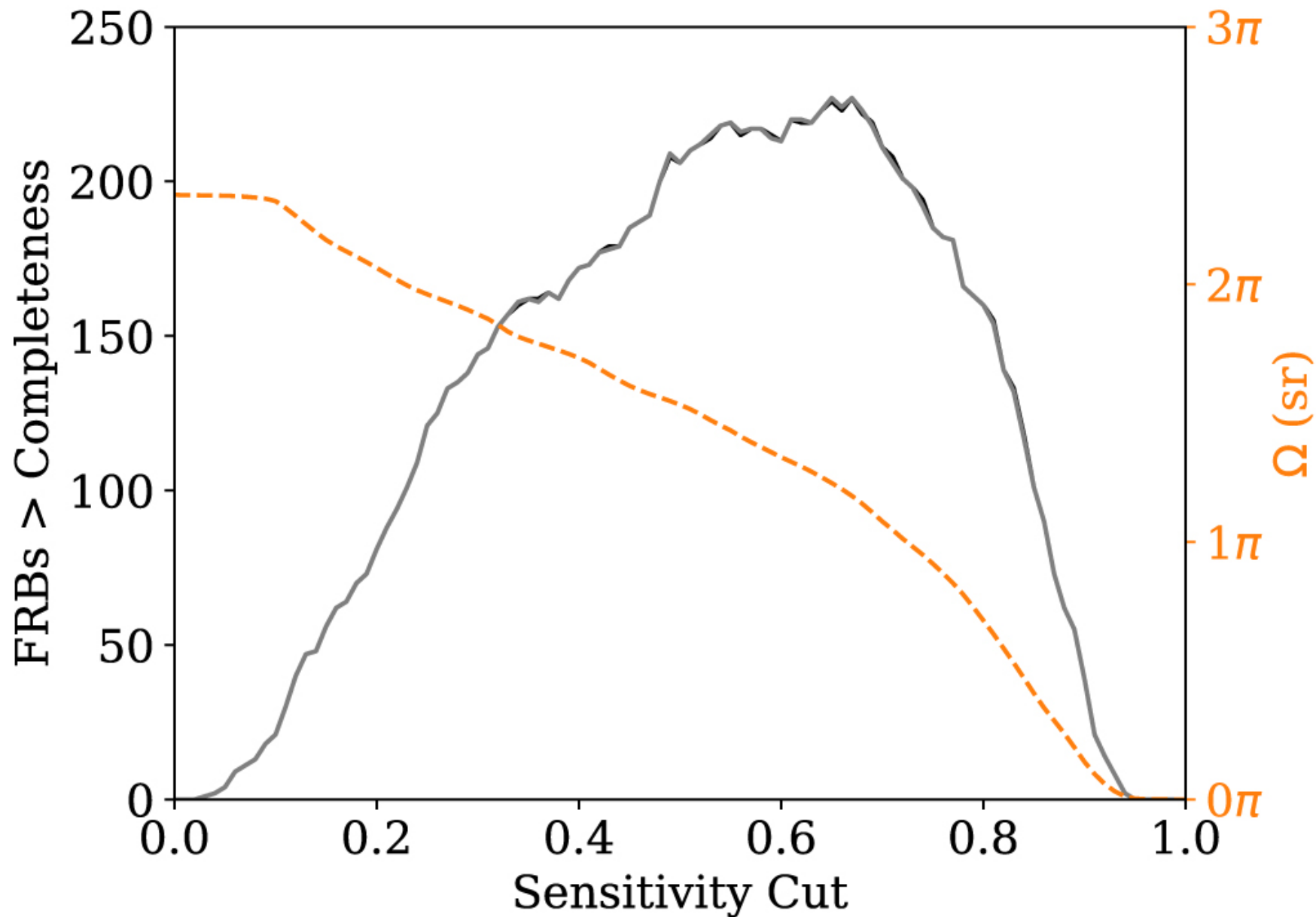
Figure 5. from No Evidence for Galactic Latitude Dependence of the Fast Radio Burst Sky Distribution null 2021 APJ 923 2 doi:10.3847/1538-4357/ac33ad https://dx.doi.org/10.3847/1538-4357/ac33ad © 2021. The Author(s). Published by the American Astronomical Society.
