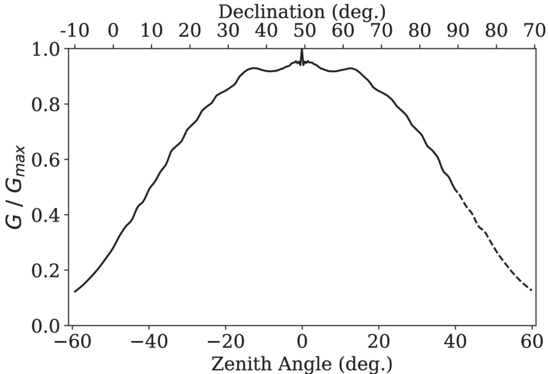
Figure 2. from No Evidence for Galactic Latitude Dependence of the Fast Radio Burst Sky Distribution null 2021 APJ 923 2 doi:10.3847/1538-4357/ac33ad https://dx.doi.org/10.3847/1538-4357/ac33ad © 2021. The Author(s). Published by the American Astronomical Society.
