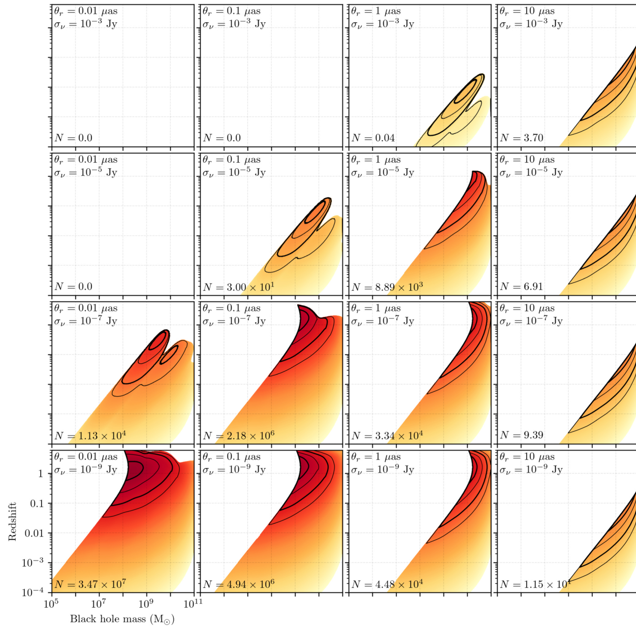
Figure 8. from Toward Determining the Number of Observable Supermassive Black Hole Shadows null 2021 APJ 923 260 doi:10.3847/1538-4357/ac2eb5 https://dx.doi.org/10.3847/1538-4357/ac2eb5 © 2021. The Author(s). Published by the American Astronomical Society.
