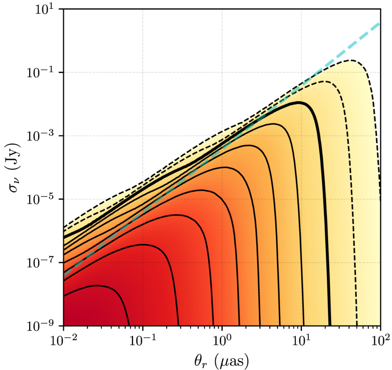
Figure 7. from Toward Determining the Number of Observable Supermassive Black Hole Shadows null 2021 APJ 923 260 doi:10.3847/1538-4357/ac2eb5 https://dx.doi.org/10.3847/1538-4357/ac2eb5 © 2021. The Author(s). Published by the American Astronomical Society.
