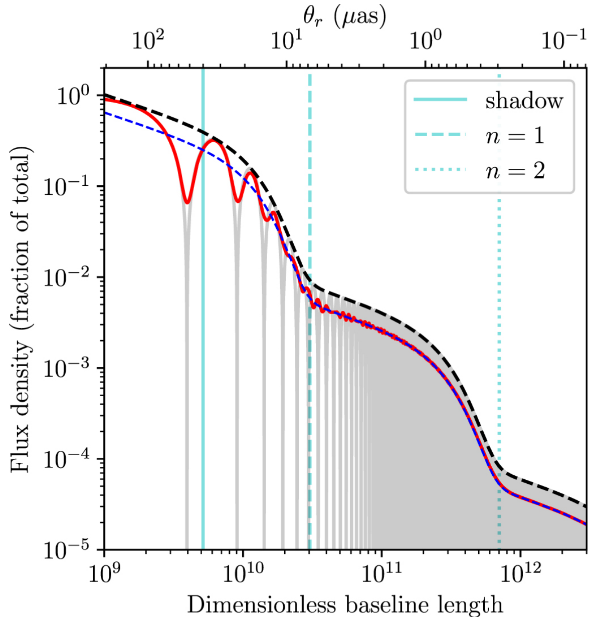
Figure 6. from Toward Determining the Number of Observable Supermassive Black Hole Shadows null 2021 APJ 923 260 doi:10.3847/1538-4357/ac2eb5 https://dx.doi.org/10.3847/1538-4357/ac2eb5 © 2021. The Author(s). Published by the American Astronomical Society.
