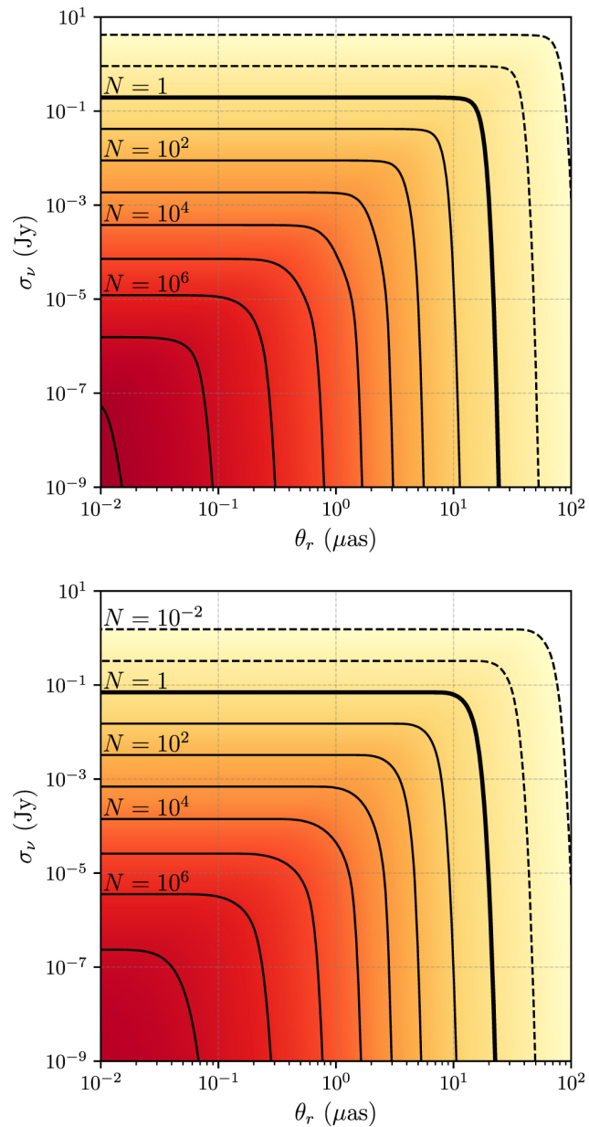
Figure 4. from Toward Determining the Number of Observable Supermassive Black Hole Shadows null 2021 APJ 923 260 doi:10.3847/1538-4357/ac2eb5 https://dx.doi.org/10.3847/1538-4357/ac2eb5 © 2021. The Author(s). Published by the American Astronomical Society.
