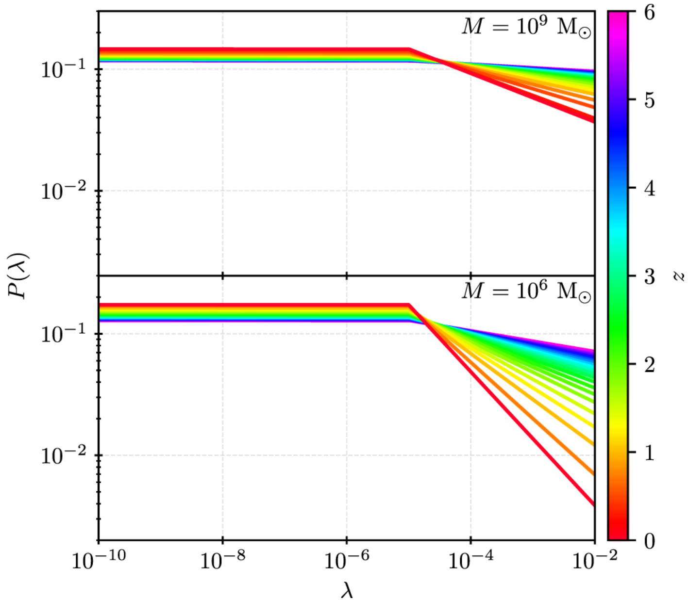
Figure 3. from Toward Determining the Number of Observable Supermassive Black Hole Shadows null 2021 APJ 923 260 doi:10.3847/1538-4357/ac2eb5 https://dx.doi.org/10.3847/1538-4357/ac2eb5 © 2021. The Author(s). Published by the American Astronomical Society.
