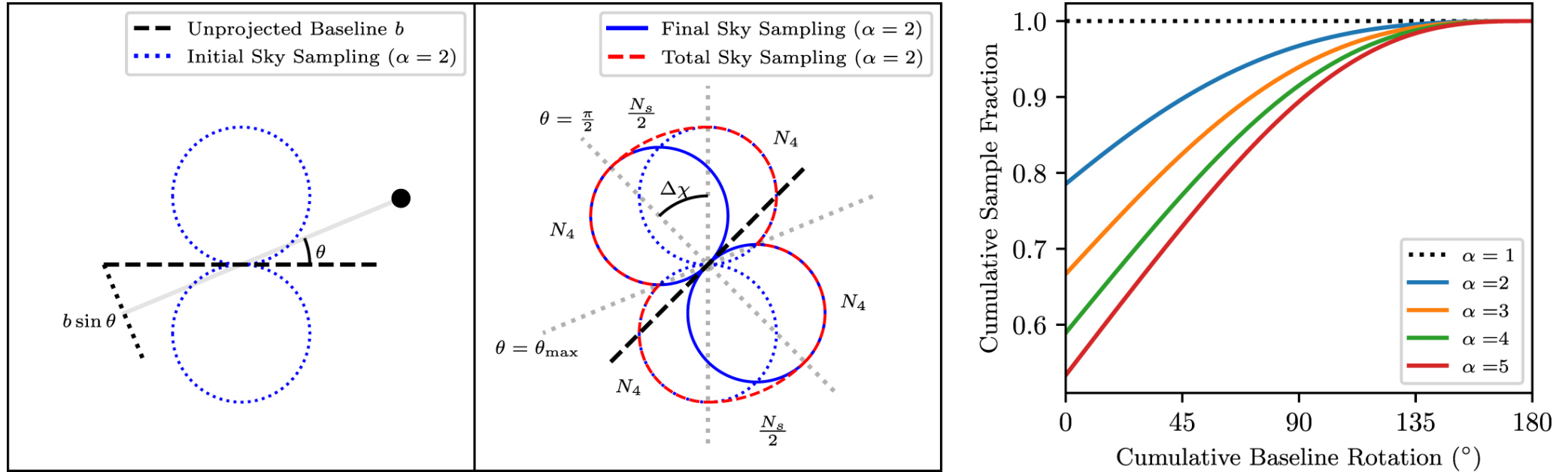
Figure 18. from Toward Determining the Number of Observable Supermassive Black Hole Shadows null 2021 APJ 923 260 doi:10.3847/1538-4357/ac2eb5 https://dx.doi.org/10.3847/1538-4357/ac2eb5 © 2021. The Author(s). Published by the American Astronomical Society.
