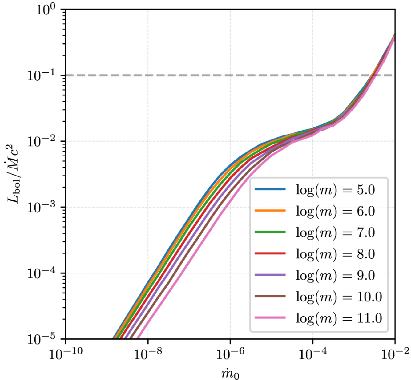
Figure 15. from Toward Determining the Number of Observable Supermassive Black Hole Shadows null 2021 APJ 923 260 doi:10.3847/1538-4357/ac2eb5 https://dx.doi.org/10.3847/1538-4357/ac2eb5 © 2021. The Author(s). Published by the American Astronomical Society.
