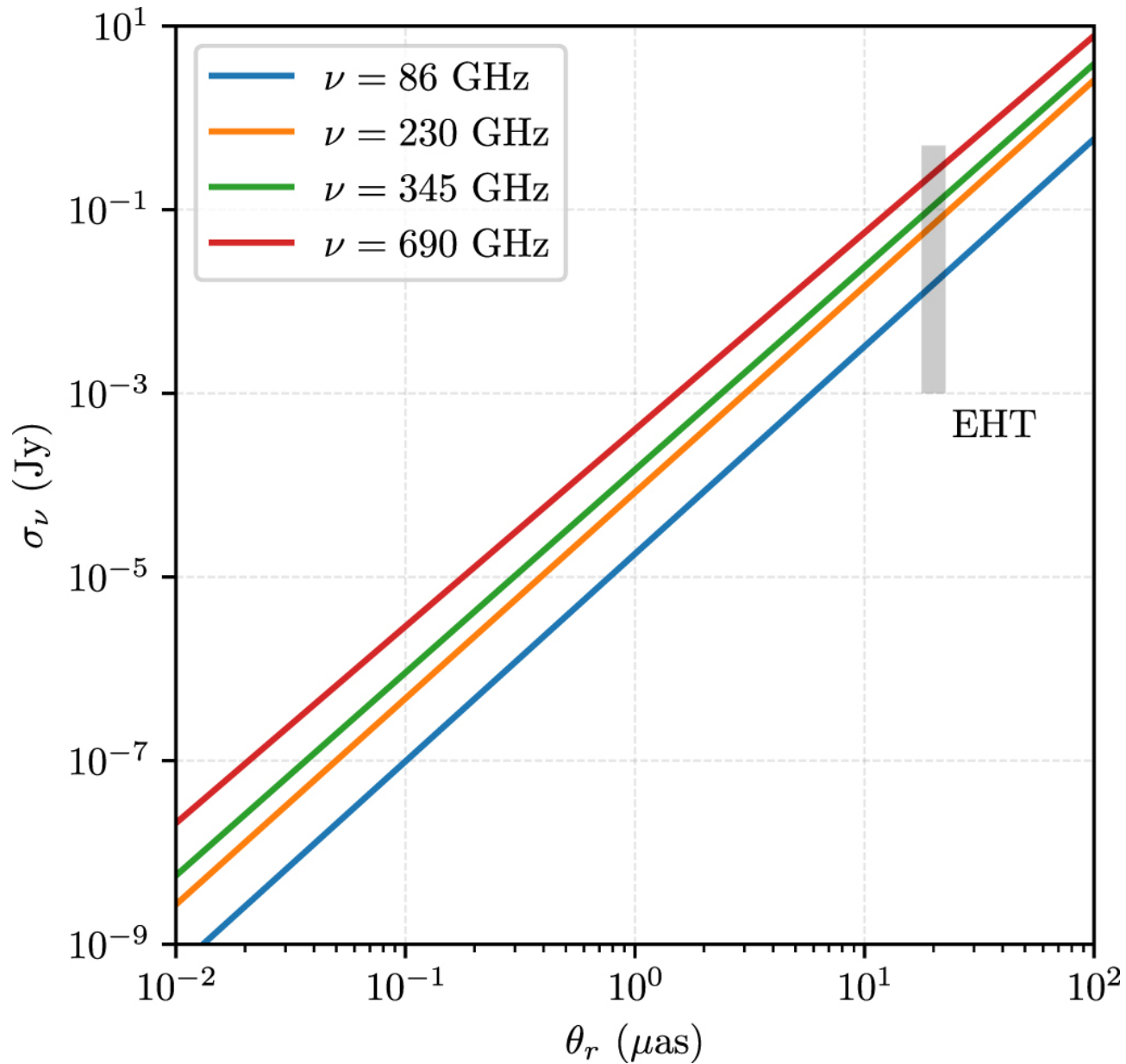
Figure 11. from Toward Determining the Number of Observable Supermassive Black Hole Shadows null 2021 APJ 923 260 doi:10.3847/1538-4357/ac2eb5 https://dx.doi.org/10.3847/1538-4357/ac2eb5 © 2021. The Author(s). Published by the American Astronomical Society.
