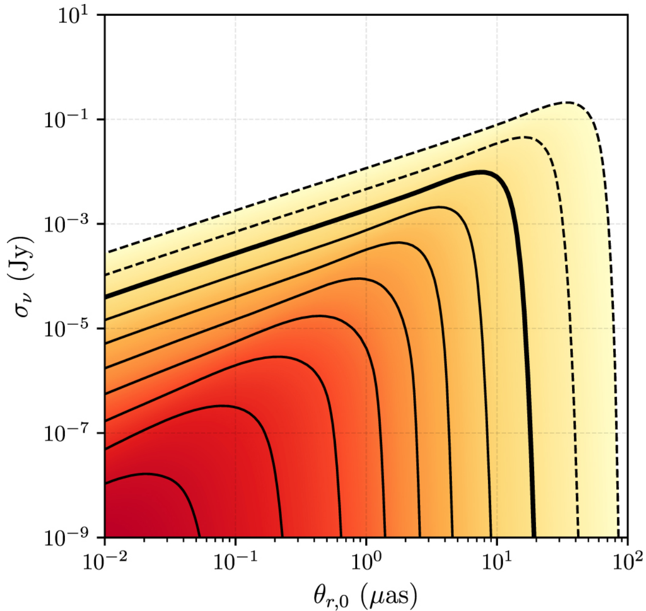
Figure 10. from Toward Determining the Number of Observable Supermassive Black Hole Shadows null 2021 APJ 923 260 doi:10.3847/1538-4357/ac2eb5 https://dx.doi.org/10.3847/1538-4357/ac2eb5 © 2021. The Author(s). Published by the American Astronomical Society.
