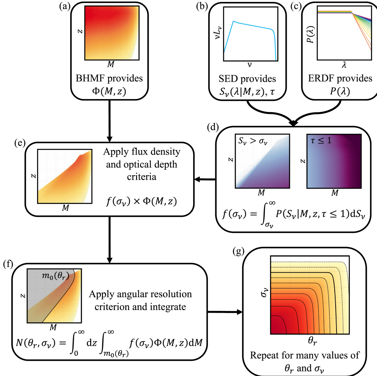
Figure 1. from Toward Determining the Number of Observable Supermassive Black Hole Shadows null 2021 APJ 923 260 doi:10.3847/1538-4357/ac2eb5 https://dx.doi.org/10.3847/1538-4357/ac2eb5 © 2021. The Author(s). Published by the American Astronomical Society.
