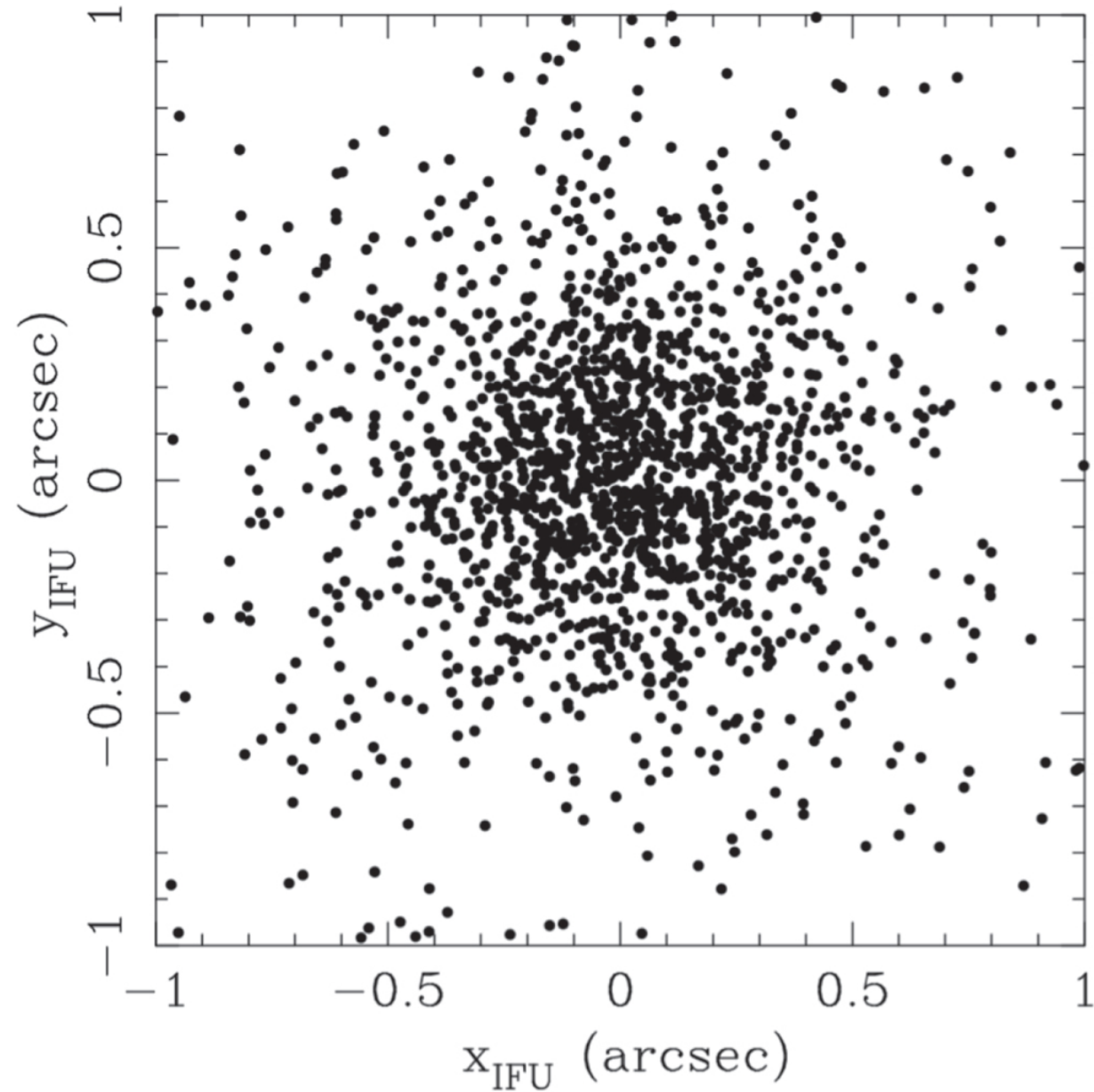
Figure 9. from The Hobby–Eberly Telescope Dark Energy Experiment (HETDEX) Survey Design, Reductions, and Detections null 2021 APJ 923 217 doi:10.3847/1538-4357/ac2e03 https://dx.doi.org/10.3847/1538-4357/ac2e03 © 2021. The Author(s). Published by the American Astronomical Society.
