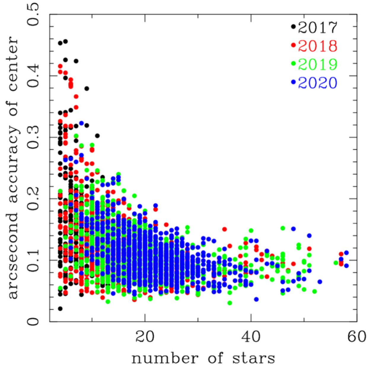
Figure 8. from The Hobby–Eberly Telescope Dark Energy Experiment (HETDEX) Survey Design, Reductions, and Detections null 2021 APJ 923 217 doi:10.3847/1538-4357/ac2e03 https://dx.doi.org/10.3847/1538-4357/ac2e03 © 2021. The Author(s). Published by the American Astronomical Society.
