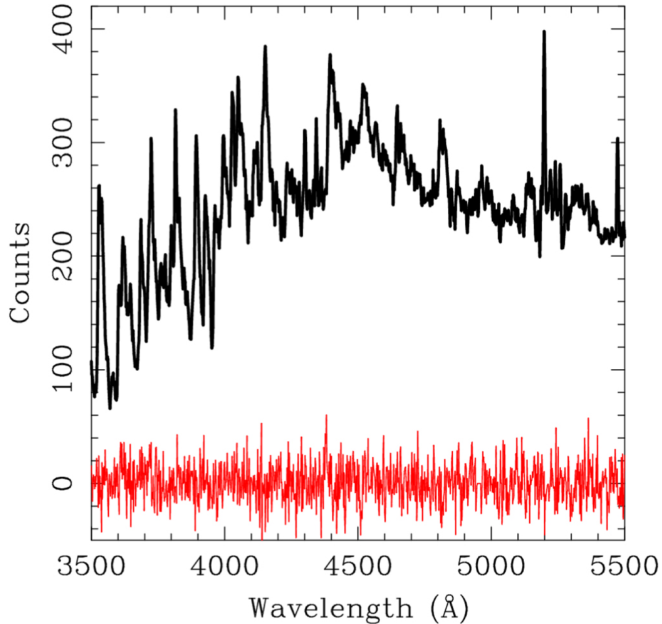
Figure 7. from The Hobby–Eberly Telescope Dark Energy Experiment (HETDEX) Survey Design, Reductions, and Detections null 2021 APJ 923 217 doi:10.3847/1538-4357/ac2e03 https://dx.doi.org/10.3847/1538-4357/ac2e03 © 2021. The Author(s). Published by the American Astronomical Society.
