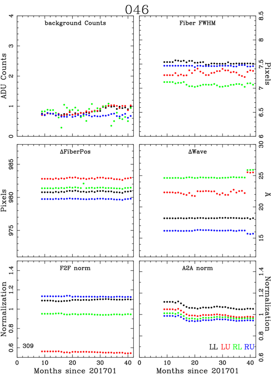
Figure 6. from The Hobby–Eberly Telescope Dark Energy Experiment (HETDEX) Survey Design, Reductions, and Detections null 2021 APJ 923 217 doi:10.3847/1538-4357/ac2e03 https://dx.doi.org/10.3847/1538-4357/ac2e03 © 2021. The Author(s). Published by the American Astronomical Society.
