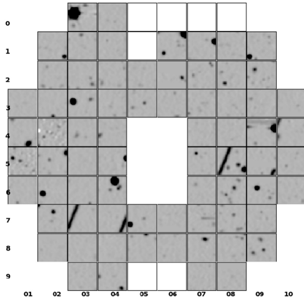
Figure 3. from The Hobby–Eberly Telescope Dark Energy Experiment (HETDEX) Survey Design, Reductions, and Detections null 2021 APJ 923 217 doi:10.3847/1538-4357/ac2e03 https://dx.doi.org/10.3847/1538-4357/ac2e03 © 2021. The Author(s). Published by the American Astronomical Society.
