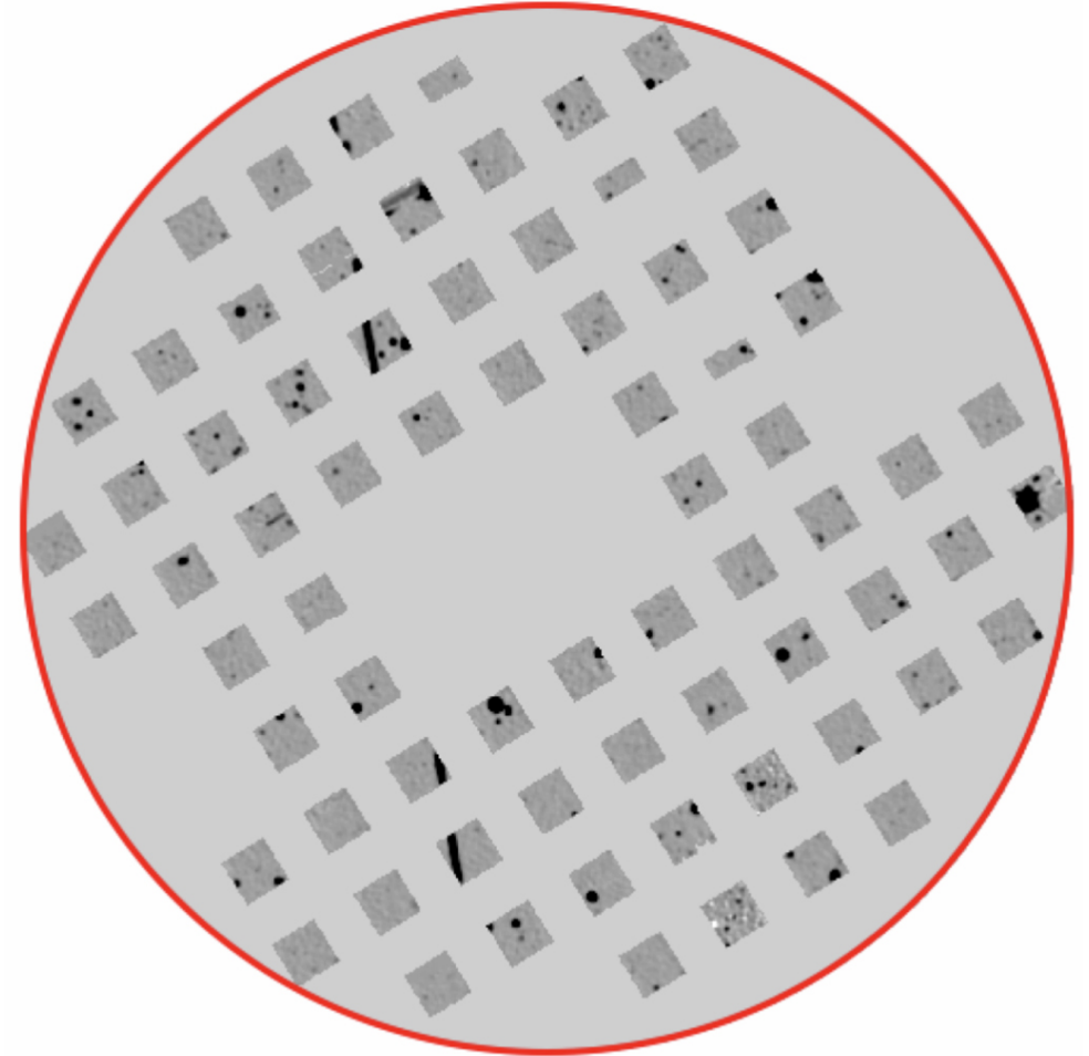
Figure 3. from The Hobby–Eberly Telescope Dark Energy Experiment (HETDEX) Survey Design, Reductions, and Detections null 2021 APJ 923 217 doi:10.3847/1538-4357/ac2e03 https://dx.doi.org/10.3847/1538-4357/ac2e03 © 2021. The Author(s). Published by the American Astronomical Society.
