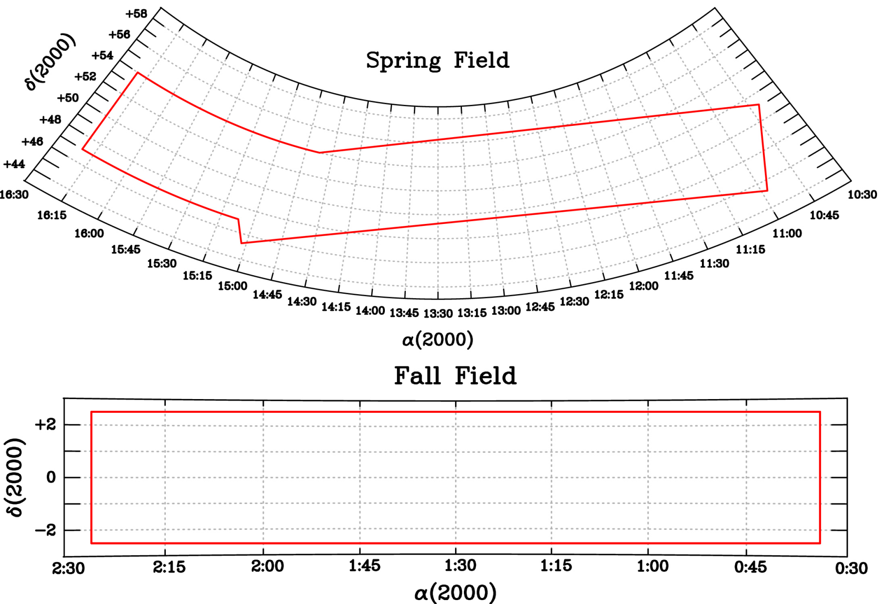
Figure 2. from The Hobby–Eberly Telescope Dark Energy Experiment (HETDEX) Survey Design, Reductions, and Detections null 2021 APJ 923 217 doi:10.3847/1538-4357/ac2e03 https://dx.doi.org/10.3847/1538-4357/ac2e03 © 2021. The Author(s). Published by the American Astronomical Society.
