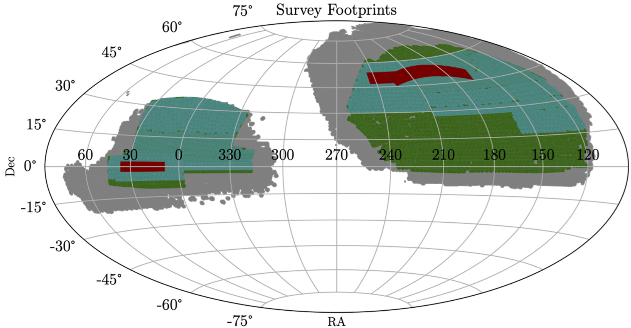
Figure 1. from The Hobby–Eberly Telescope Dark Energy Experiment (HETDEX) Survey Design, Reductions, and Detections null 2021 APJ 923 217 doi:10.3847/1538-4357/ac2e03 https://dx.doi.org/10.3847/1538-4357/ac2e03 © 2021. The Author(s). Published by the American Astronomical Society.
