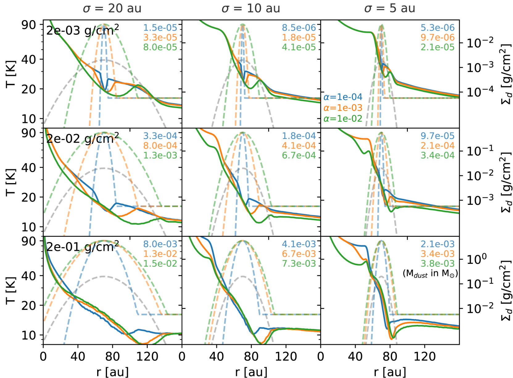
Figure 6. from Self-consistent Ring Model in Protoplanetary Disks: Temperature Dips and Substructure Formation null 2021 APJ 923 70 doi:10.3847/1538-4357/ac2c82 https://dx.doi.org/10.3847/1538-4357/ac2c82 © 2021. The American Astronomical Society. All rights reserved.
