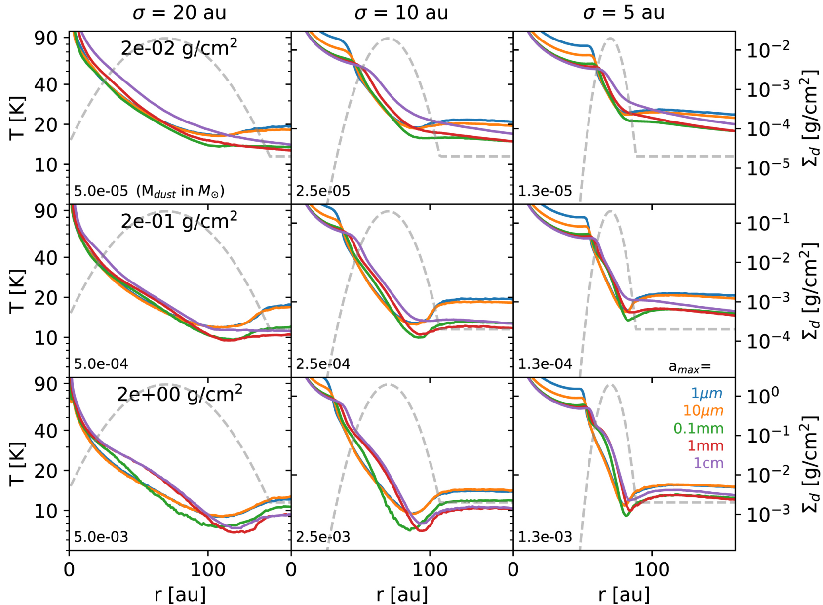
Figure 5. from Self-consistent Ring Model in Protoplanetary Disks: Temperature Dips and Substructure Formation null 2021 APJ 923 70 doi:10.3847/1538-4357/ac2c82 https://dx.doi.org/10.3847/1538-4357/ac2c82 © 2021. The American Astronomical Society. All rights reserved.
