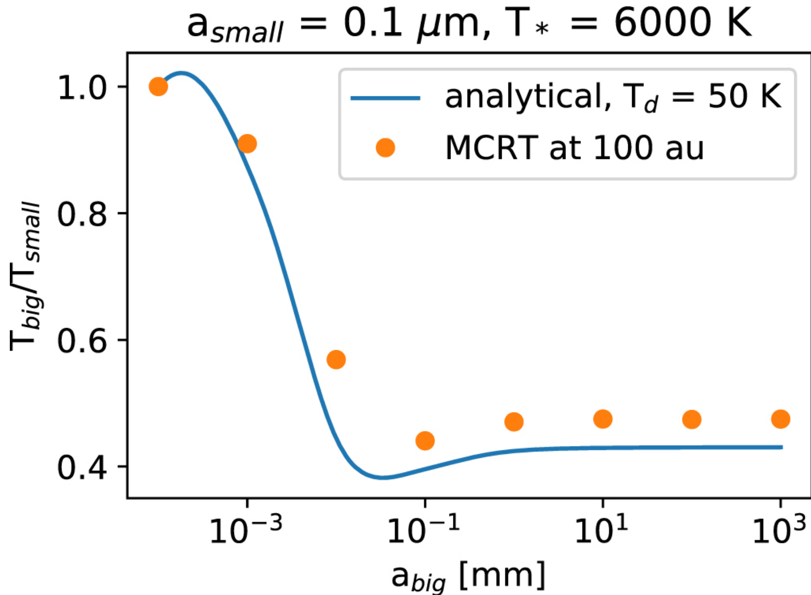
Figure 3. from Self-consistent Ring Model in Protoplanetary Disks: Temperature Dips and Substructure Formation null 2021 APJ 923 70 doi:10.3847/1538-4357/ac2c82 https://dx.doi.org/10.3847/1538-4357/ac2c82 © 2021. The American Astronomical Society. All rights reserved.
