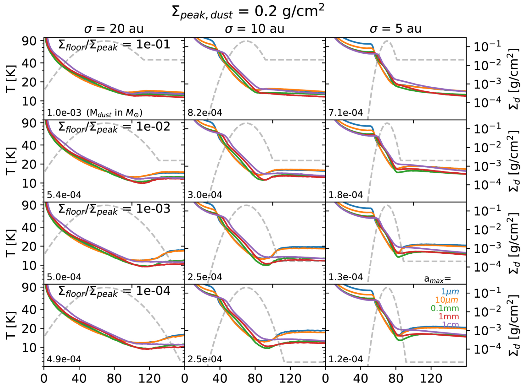
Figure 11. from Self-consistent Ring Model in Protoplanetary Disks: Temperature Dips and Substructure Formation null 2021 APJ 923 70 doi:10.3847/1538-4357/ac2c82 https://dx.doi.org/10.3847/1538-4357/ac2c82 © 2021. The American Astronomical Society. All rights reserved.
