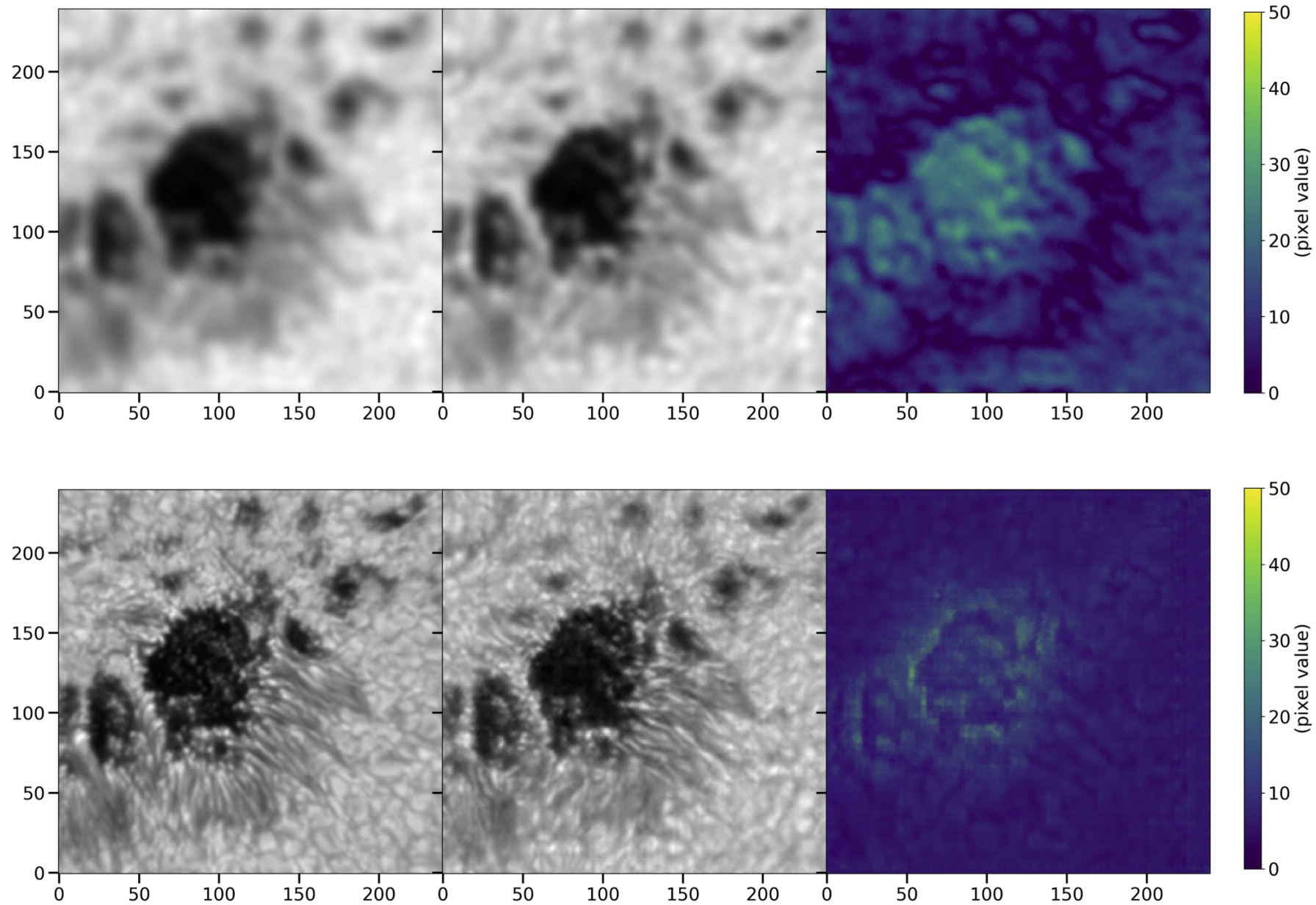
Figure 8. from Improving the Spatial Resolution of Solar Images Using Generative Adversarial Network and Self-attention Mechanism null 2021 APJ 923 76 doi:10.3847/1538-4357/ac2aa2 https://dx.doi.org/10.3847/1538-4357/ac2aa2 © 2021. The American Astronomical Society. All rights reserved.
