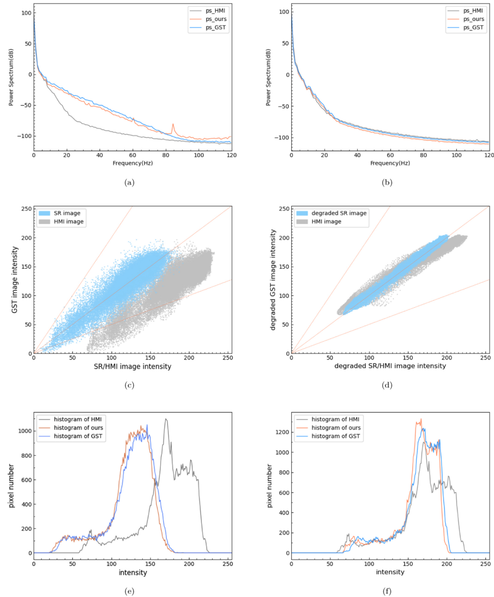
Figure 7. from Improving the Spatial Resolution of Solar Images Using Generative Adversarial Network and Self-attention Mechanism null 2021 APJ 923 76 doi:10.3847/1538-4357/ac2aa2 https://dx.doi.org/10.3847/1538-4357/ac2aa2 © 2021. The American Astronomical Society. All rights reserved.
