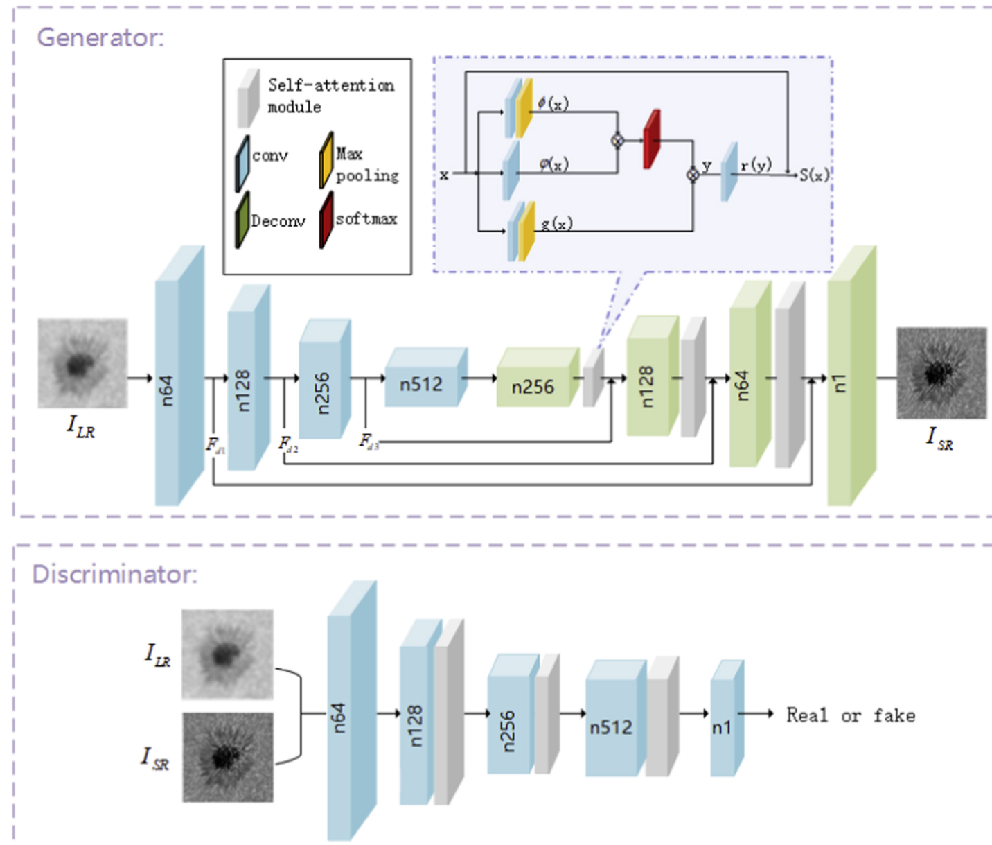
Figure 2. from Improving the Spatial Resolution of Solar Images Using Generative Adversarial Network and Self-attention Mechanism null 2021 APJ 923 76 doi:10.3847/1538-4357/ac2aa2 https://dx.doi.org/10.3847/1538-4357/ac2aa2 © 2021. The American Astronomical Society. All rights reserved.
