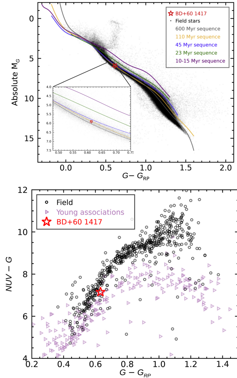
Figure 9. from A Wide Planetary Mass Companion Discovered through the Citizen Science Project Backyard Worlds: Planet 9 null 2021 APJ 923 48 doi:10.3847/1538-4357/ac2499 https://dx.doi.org/10.3847/1538-4357/ac2499 © 2021. The American Astronomical Society. All rights reserved.
