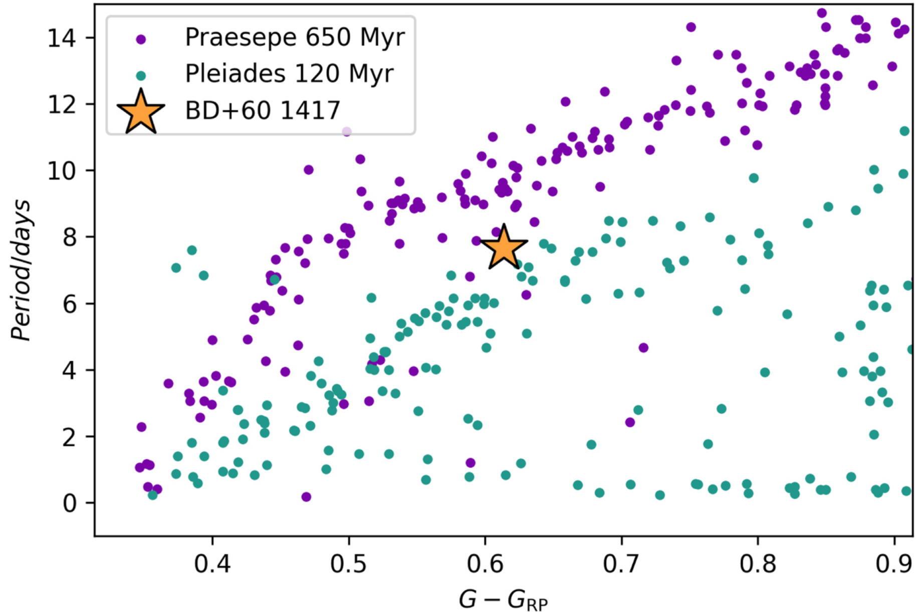
Figure 8. from A Wide Planetary Mass Companion Discovered through the Citizen Science Project Backyard Worlds: Planet 9 null 2021 APJ 923 48 doi:10.3847/1538-4357/ac2499 https://dx.doi.org/10.3847/1538-4357/ac2499 © 2021. The American Astronomical Society. All rights reserved.
