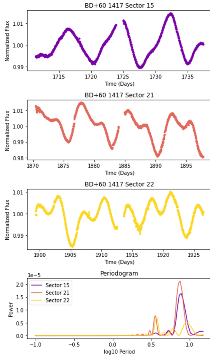
Figure 7. from A Wide Planetary Mass Companion Discovered through the Citizen Science Project Backyard Worlds: Planet 9 null 2021 APJ 923 48 doi:10.3847/1538-4357/ac2499 https://dx.doi.org/10.3847/1538-4357/ac2499 © 2021. The American Astronomical Society. All rights reserved.
