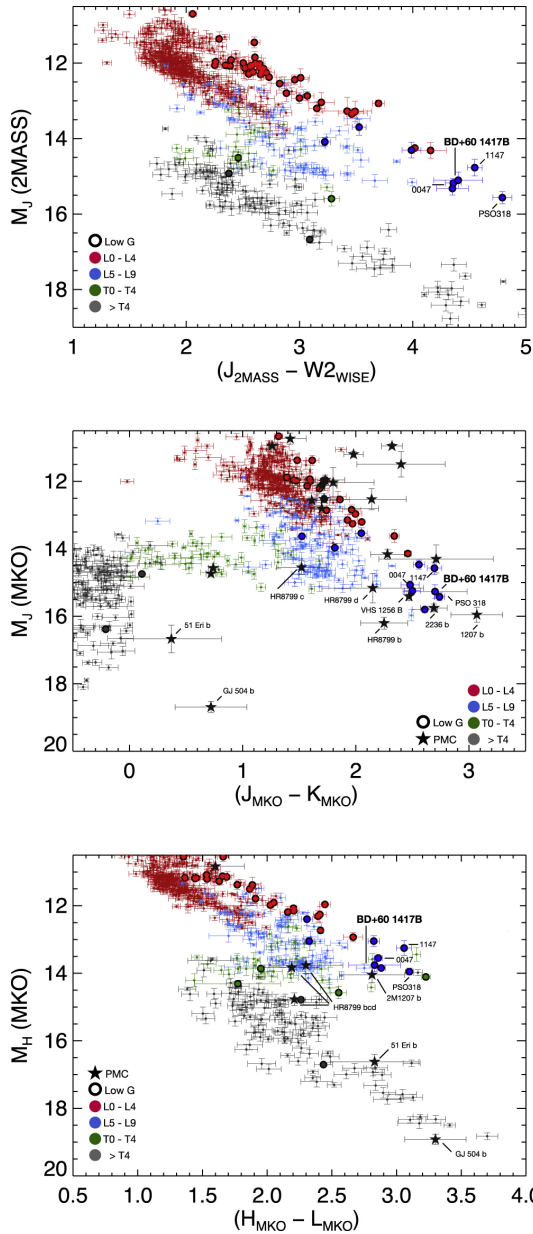
Figure 5. from A Wide Planetary Mass Companion Discovered through the Citizen Science Project Backyard Worlds: Planet 9 null 2021 APJ 923 48 doi:10.3847/1538-4357/ac2499 https://dx.doi.org/10.3847/1538-4357/ac2499 © 2021. The American Astronomical Society. All rights reserved.
