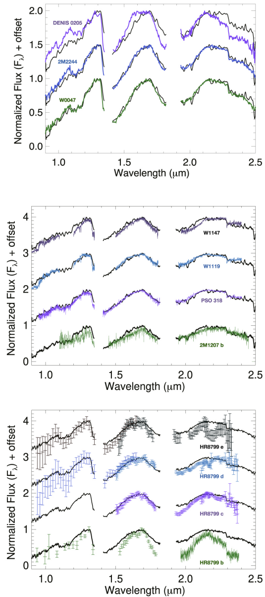
Figure 4. from A Wide Planetary Mass Companion Discovered through the Citizen Science Project Backyard Worlds: Planet 9 null 2021 APJ 923 48 doi:10.3847/1538-4357/ac2499 https://dx.doi.org/10.3847/1538-4357/ac2499 © 2021. The American Astronomical Society. All rights reserved.
