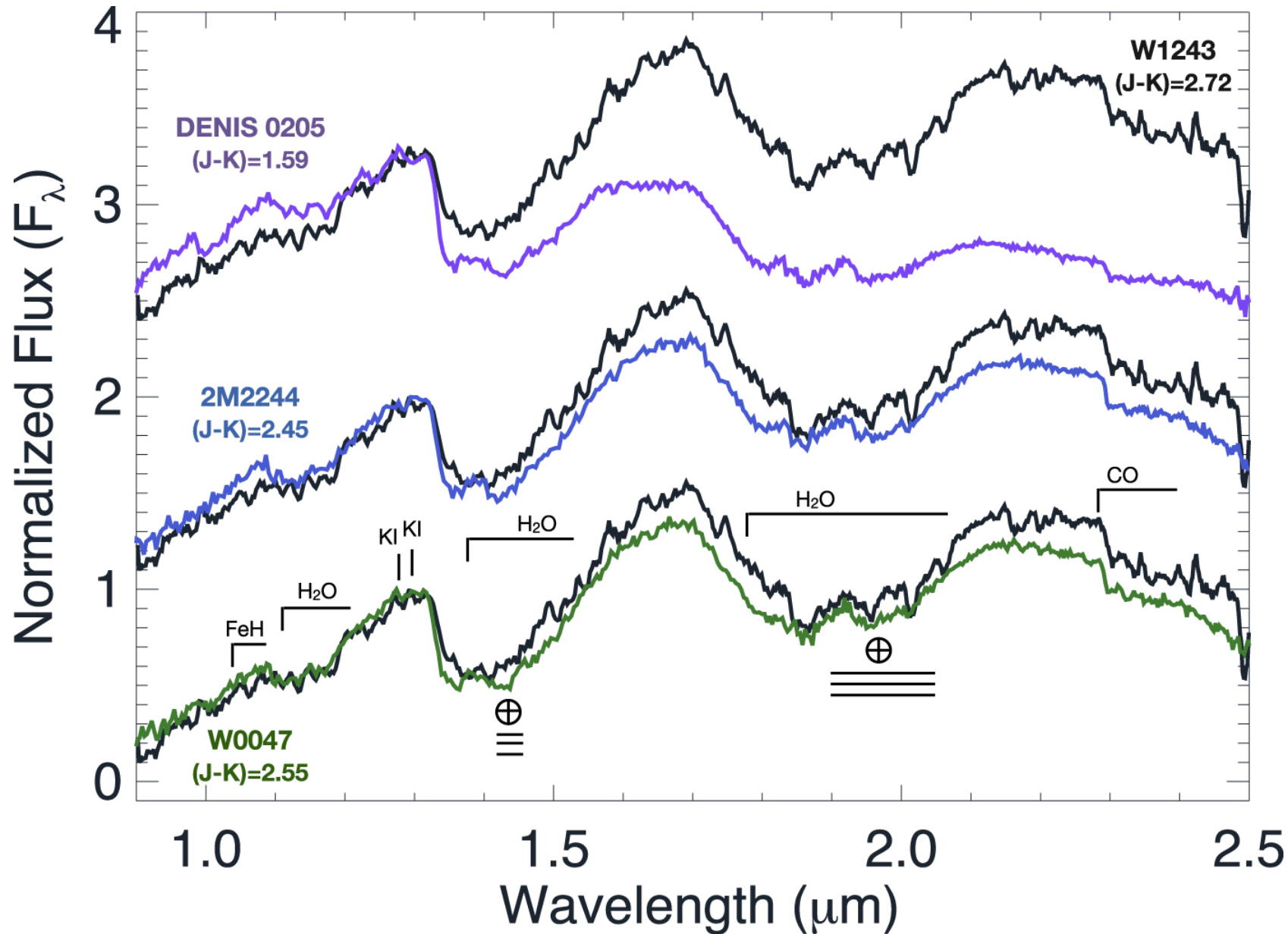
Figure 3. from A Wide Planetary Mass Companion Discovered through the Citizen Science Project Backyard Worlds: Planet 9 null 2021 APJ 923 48 doi:10.3847/1538-4357/ac2499 https://dx.doi.org/10.3847/1538-4357/ac2499 © 2021. The American Astronomical Society. All rights reserved.
