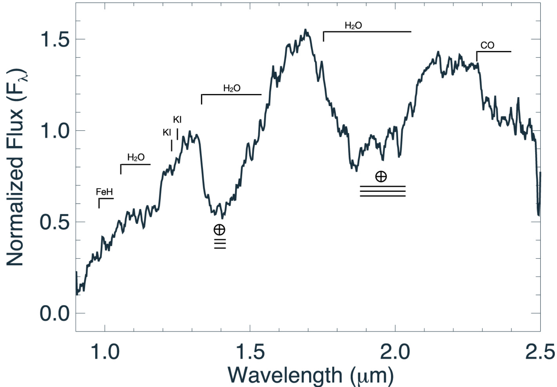
Figure 2. from A Wide Planetary Mass Companion Discovered through the Citizen Science Project Backyard Worlds: Planet 9 null 2021 APJ 923 48 doi:10.3847/1538-4357/ac2499 https://dx.doi.org/10.3847/1538-4357/ac2499 © 2021. The American Astronomical Society. All rights reserved.
