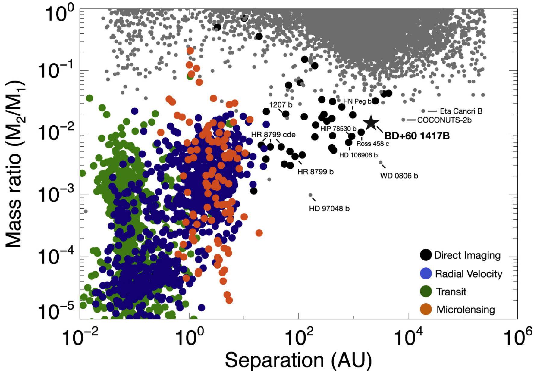
Figure 10. from A Wide Planetary Mass Companion Discovered through the Citizen Science Project Backyard Worlds: Planet 9 null 2021 APJ 923 48 doi:10.3847/1538-4357/ac2499 https://dx.doi.org/10.3847/1538-4357/ac2499 © 2021. The American Astronomical Society. All rights reserved.
