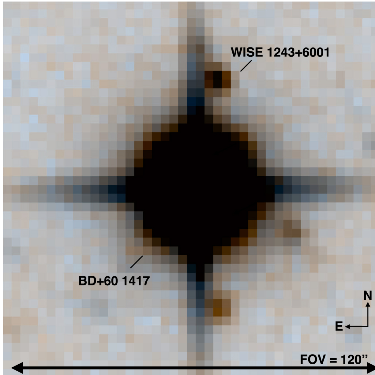
Figure 1. from A Wide Planetary Mass Companion Discovered through the Citizen Science Project Backyard Worlds: Planet 9 null 2021 APJ 923 48 doi:10.3847/1538-4357/ac2499 https://dx.doi.org/10.3847/1538-4357/ac2499 © 2021. The American Astronomical Society. All rights reserved.
