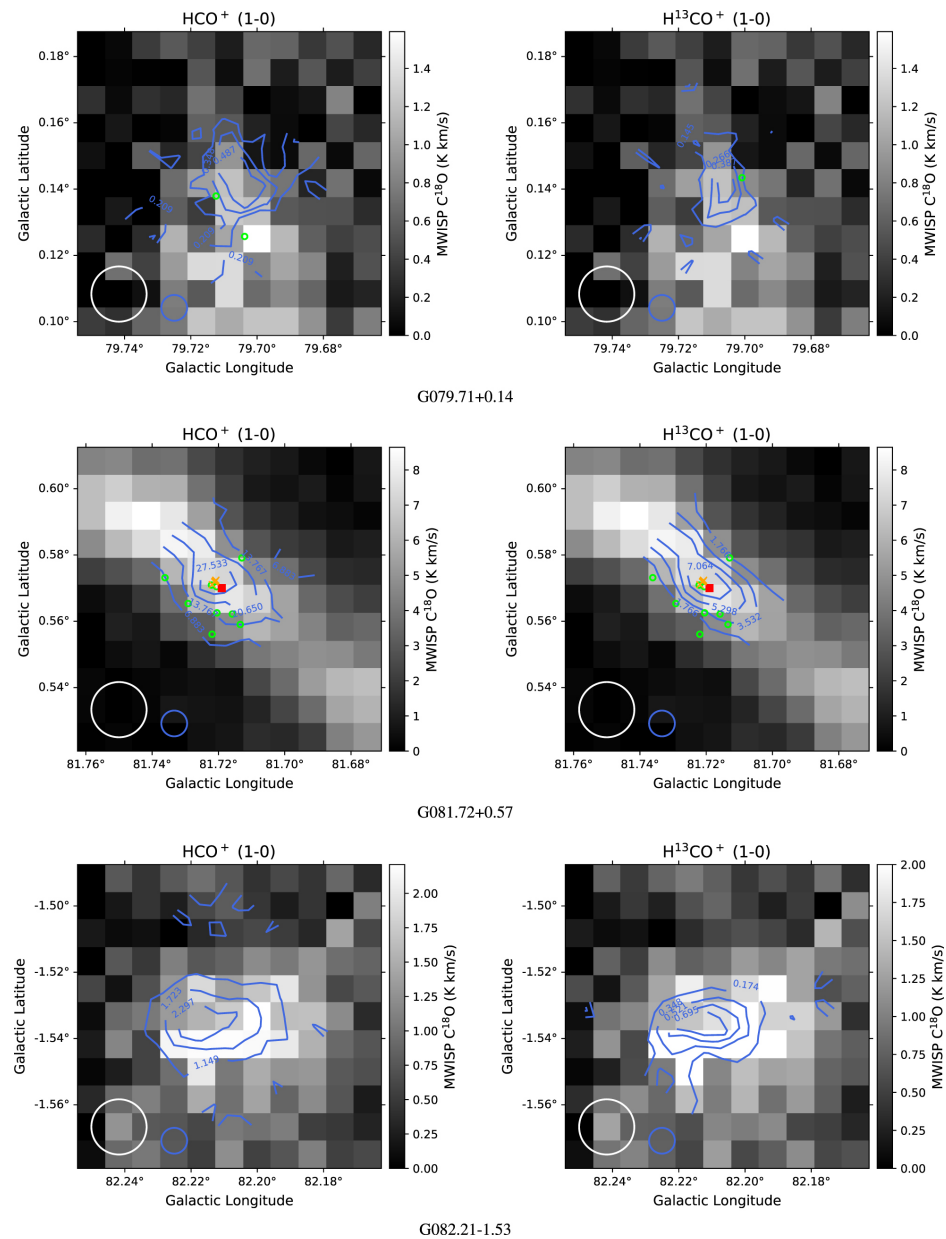
Figure A1. from Yang Yang et al 2021 Astrophys. J. 922 doi:10.3847/1538-4357/ac22ab https://dx.doi.org/10.3847/1538-4357/ac22ab © 2021. The American Astronomical Society. All rights reserved.
