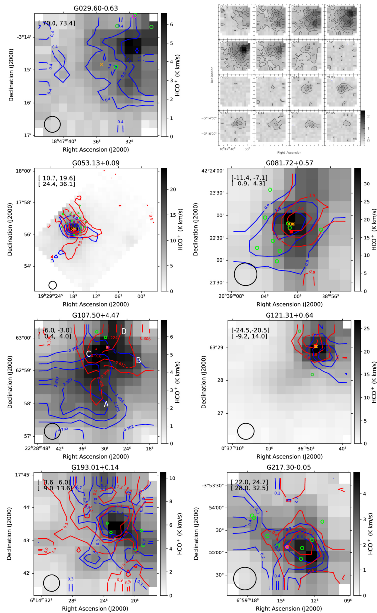
Figure 5. from Yang Yang et al 2021 Astrophys. J. 922 doi:10.3847/1538-4357/ac22ab https://dx.doi.org/10.3847/1538-4357/ac22ab © 2021. The American Astronomical Society. All rights reserved.
