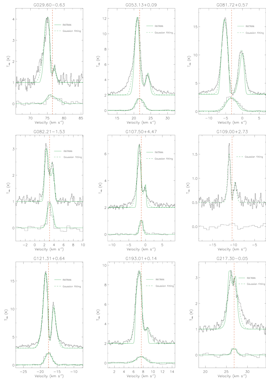
Figure 4. from Yang Yang et al 2021 Astrophys. J. 922 doi:10.3847/1538-4357/ac22ab https://dx.doi.org/10.3847/1538-4357/ac22ab © 2021. The American Astronomical Society. All rights reserved.
