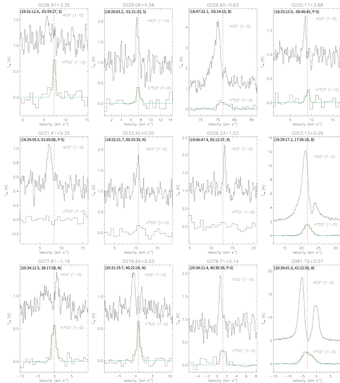
Figure 3. from Yang Yang et al 2021 Astrophys. J. 922 doi:10.3847/1538-4357/ac22ab https://dx.doi.org/10.3847/1538-4357/ac22ab © 2021. The American Astronomical Society. All rights reserved.
