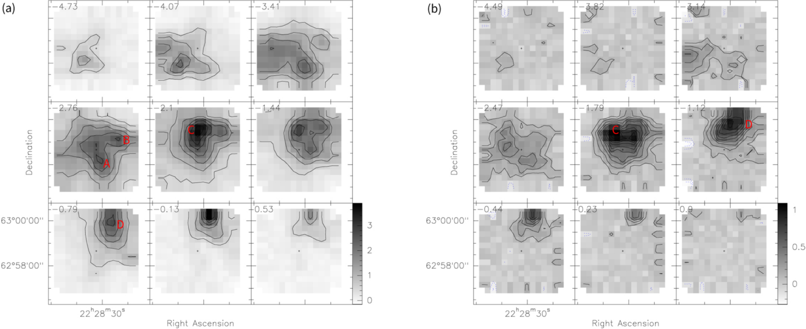
Figure 2. from Yang Yang et al 2021 Astrophys. J. 922 doi:10.3847/1538-4357/ac22ab https://dx.doi.org/10.3847/1538-4357/ac22ab © 2021. The American Astronomical Society. All rights reserved.
