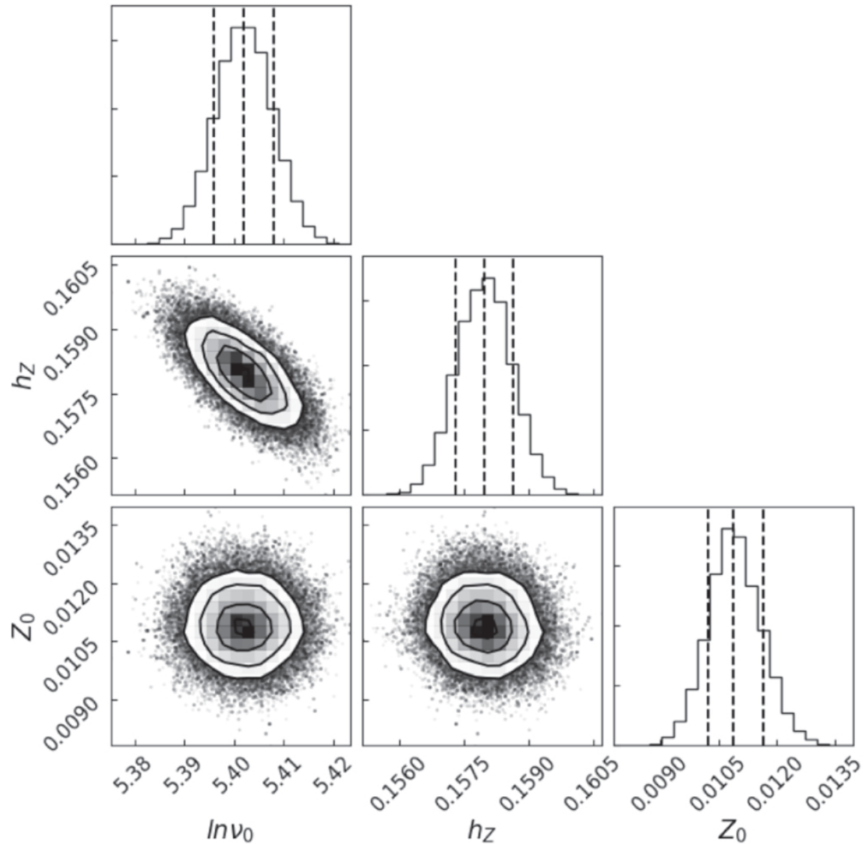
Figure 8. from Yang Yu et al 2021 Astrophys. J. 922 doi:10.3847/1538-4357/ac1e91 https://dx.doi.org/10.3847/1538-4357/ac1e91 © 2021. The American Astronomical Society. All rights reserved.
