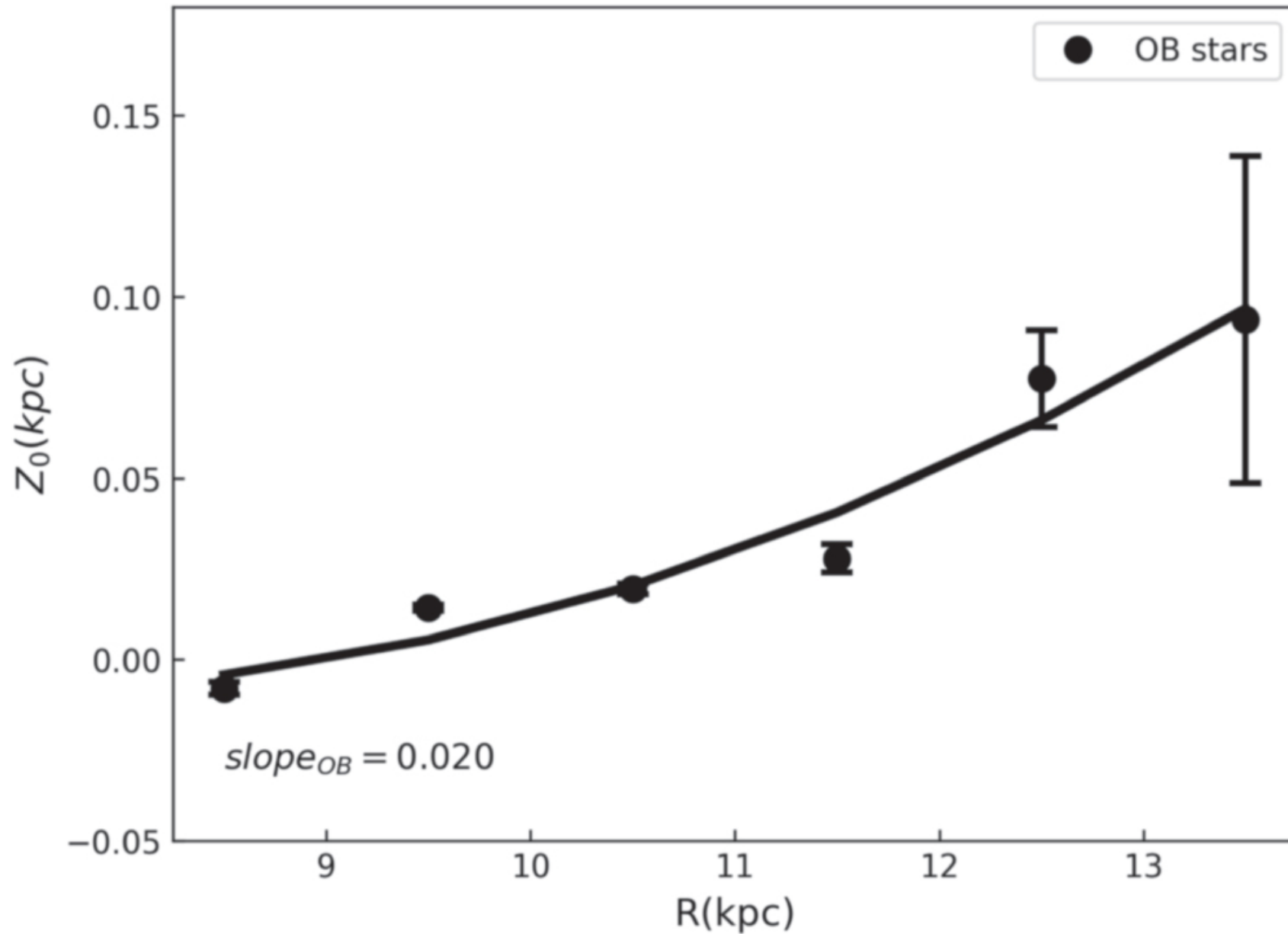
Figure 6. from Yang Yu et al 2021 Astrophys. J. 922 doi:10.3847/1538-4357/ac1e91 https://dx.doi.org/10.3847/1538-4357/ac1e91 © 2021. The American Astronomical Society. All rights reserved.
