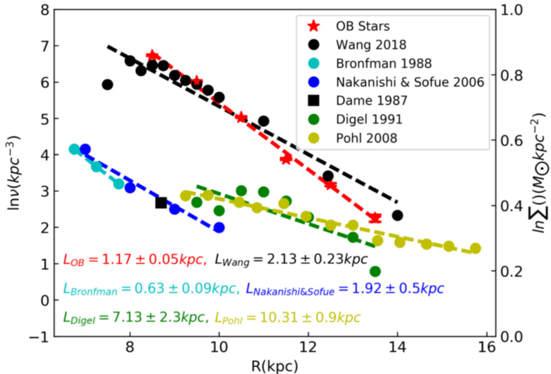
Figure 5. from Yang Yu et al 2021 Astrophys. J. 922 doi:10.3847/1538-4357/ac1e91 https://dx.doi.org/10.3847/1538-4357/ac1e91 © 2021. The American Astronomical Society. All rights reserved.
