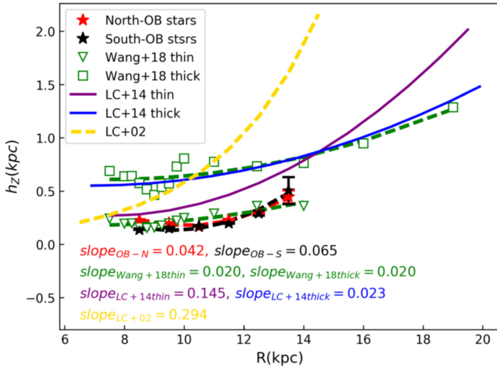
Figure 3. from Yang Yu et al 2021 Astrophys. J. 922 doi:10.3847/1538-4357/ac1e91 https://dx.doi.org/10.3847/1538-4357/ac1e91 © 2021. The American Astronomical Society. All rights reserved.
