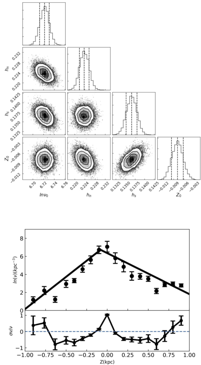
Figure 2. from Yang Yu et al 2021 Astrophys. J. 922 doi:10.3847/1538-4357/ac1e91 https://dx.doi.org/10.3847/1538-4357/ac1e91 © 2021. The American Astronomical Society. All rights reserved.
