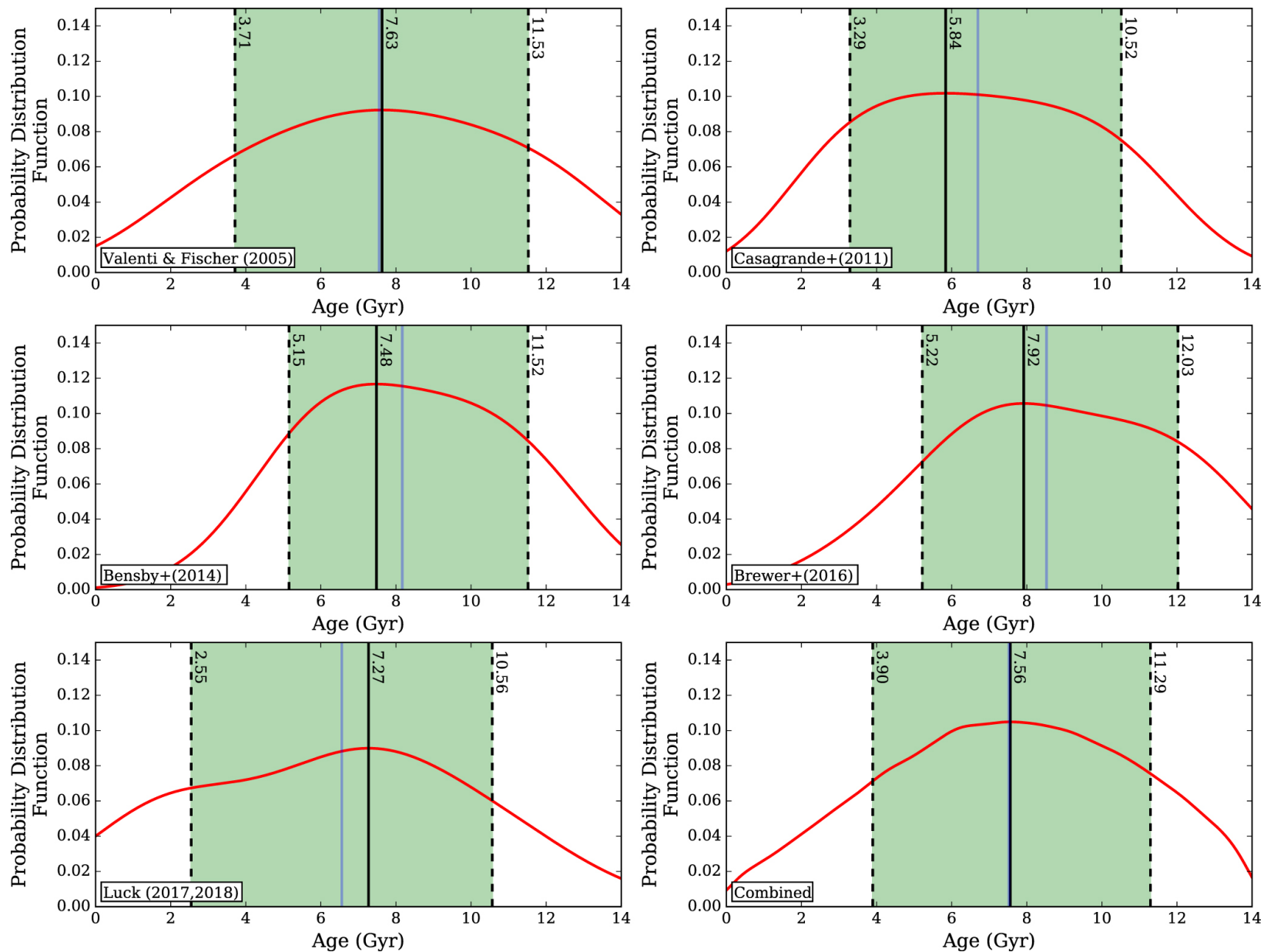
Figure 7. from Adam C. Schneider et al 2021 Astrophys. J. 921 doi:10.3847/1538-4357/ac1c75 https://dx.doi.org/10.3847/1538-4357/ac1c75 © 2021. The American Astronomical Society. All rights reserved.
