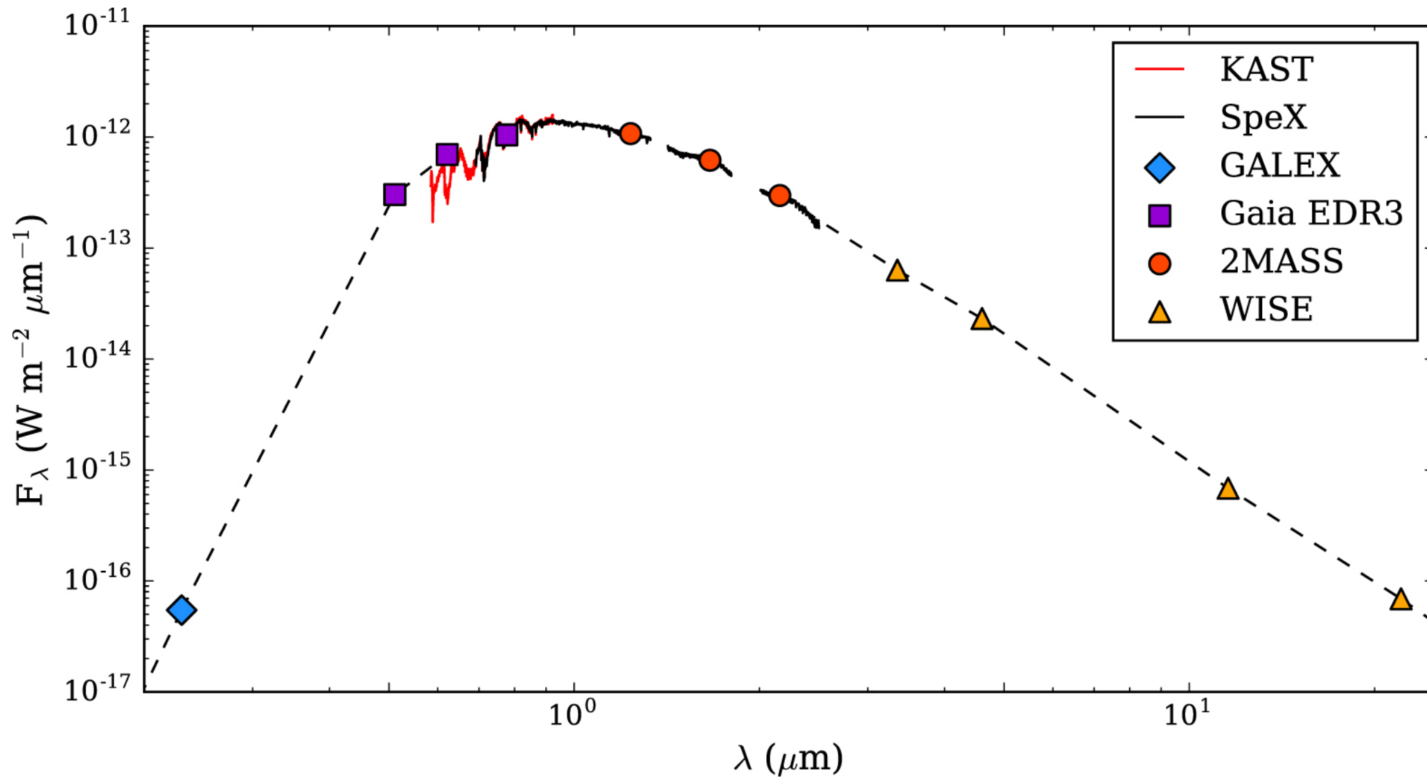
Figure 6. from Adam C. Schneider et al 2021 Astrophys. J. 921 doi:10.3847/1538-4357/ac1c75 https://dx.doi.org/10.3847/1538-4357/ac1c75 © 2021. The American Astronomical Society. All rights reserved.
