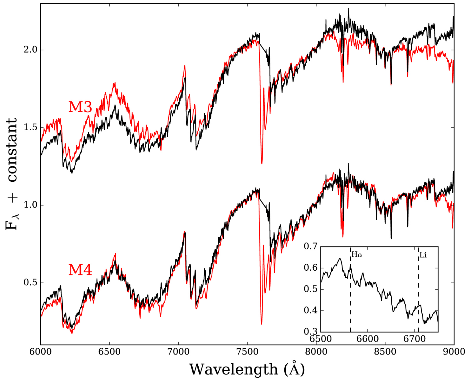
Figure 5. from Adam C. Schneider et al 2021 Astrophys. J. 921 doi:10.3847/1538-4357/ac1c75 https://dx.doi.org/10.3847/1538-4357/ac1c75 © 2021. The American Astronomical Society. All rights reserved.
