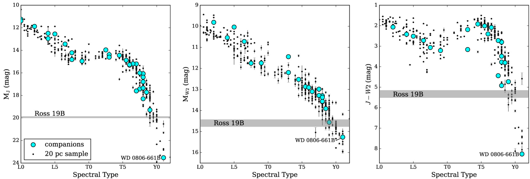
Figure 4. from Adam C. Schneider et al 2021 Astrophys. J. 921 doi:10.3847/1538-4357/ac1c75 https://dx.doi.org/10.3847/1538-4357/ac1c75 © 2021. The American Astronomical Society. All rights reserved.
