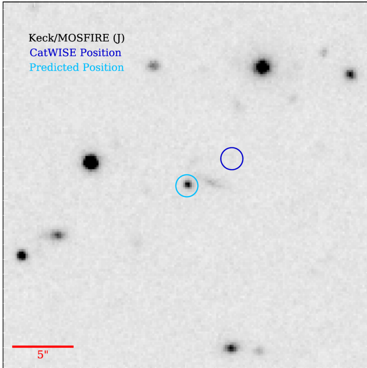
Figure 2. from Adam C. Schneider et al 2021 Astrophys. J. 921 doi:10.3847/1538-4357/ac1c75 https://dx.doi.org/10.3847/1538-4357/ac1c75 © 2021. The American Astronomical Society. All rights reserved.
